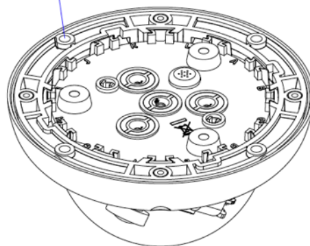
Mounting ring
